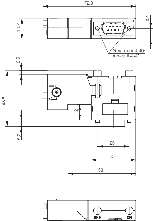
Profibus without PU connection
