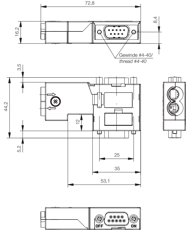
Profibus with PU connection
